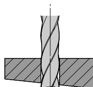
Reduce feed by 30% until full diameter cut or use pilot
