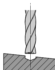
Pilot on all surfaces. No feed reduction
