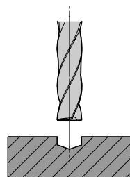
Rough or hardened surfaces, No feed reduction
